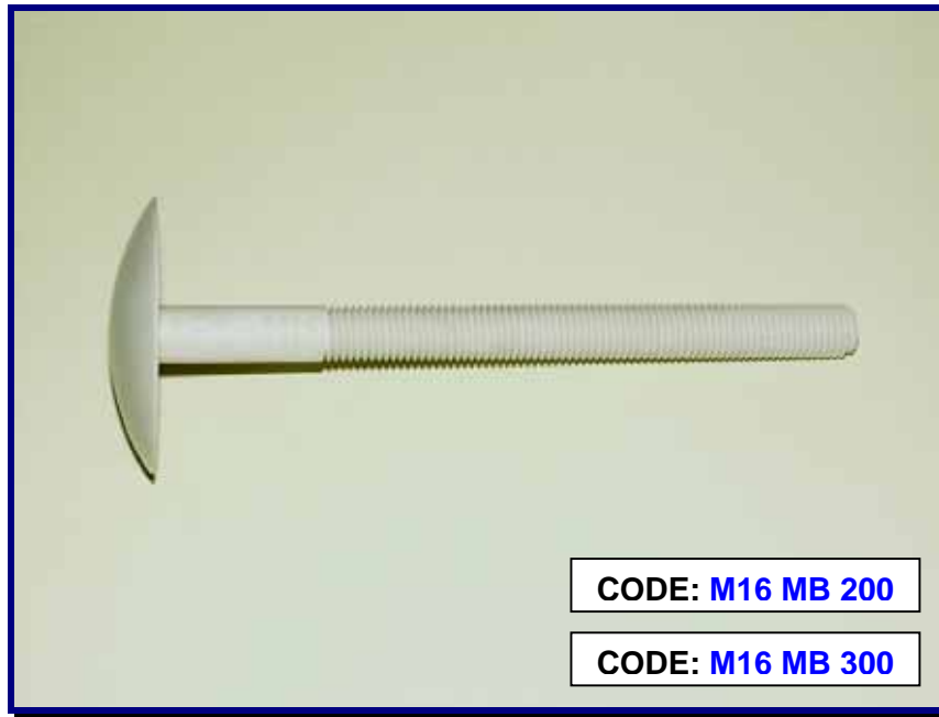
M16 Mushroom Bolt, Polyplas / Nylon Available: 200mm or 300mm Length
