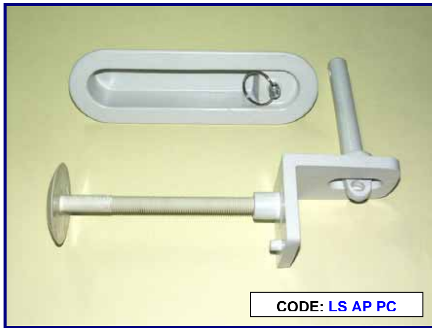
Locking System Kit, Polyplas, Alloy Pocket, Hasp, Release Pin (Offset Holes) & Keyring / Powder Coated, M16 x 300 Mushroom Bolt
