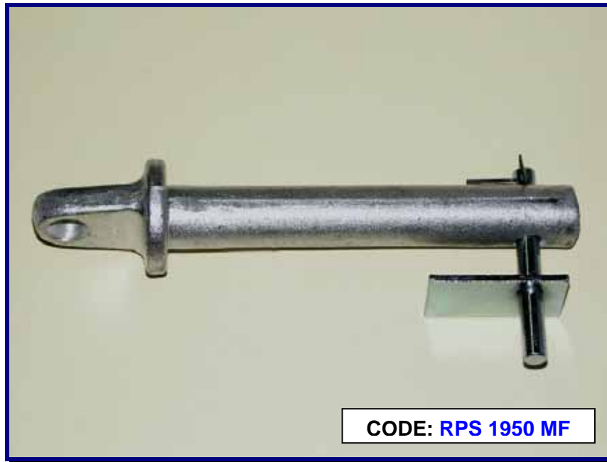
Release Pin (Inline Holes) & Swivel, Polyplas / Mill Finish Available: Mill or Powder Coated Finish Used with Plastic Pocket
