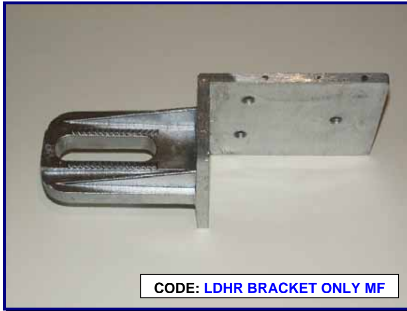
Wheel Bracket Only, Polyplas, Large Door Hanging Roller, Right Hand / Mill Finish Available: Right or Left / Mill or Powder Coated Finish
