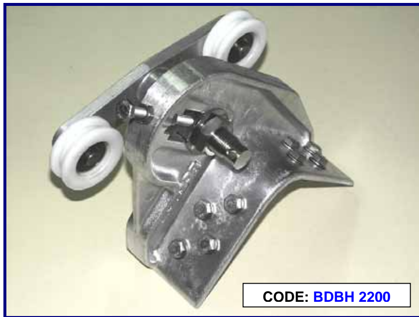
Wheel Bracket, BonDor, Double Bogie Door Hanger Roller Assembly, 55mm OD Wheels / Mill Finish, Stainless Steel Parts Available: Right or Left
