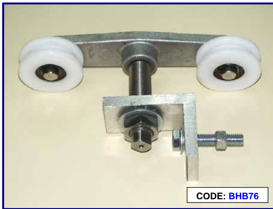
Roller Assembly, BonDor, Double Bogey 55mm OD Wheel - Mill & Alloy Finish, Stainless Steel Parts
