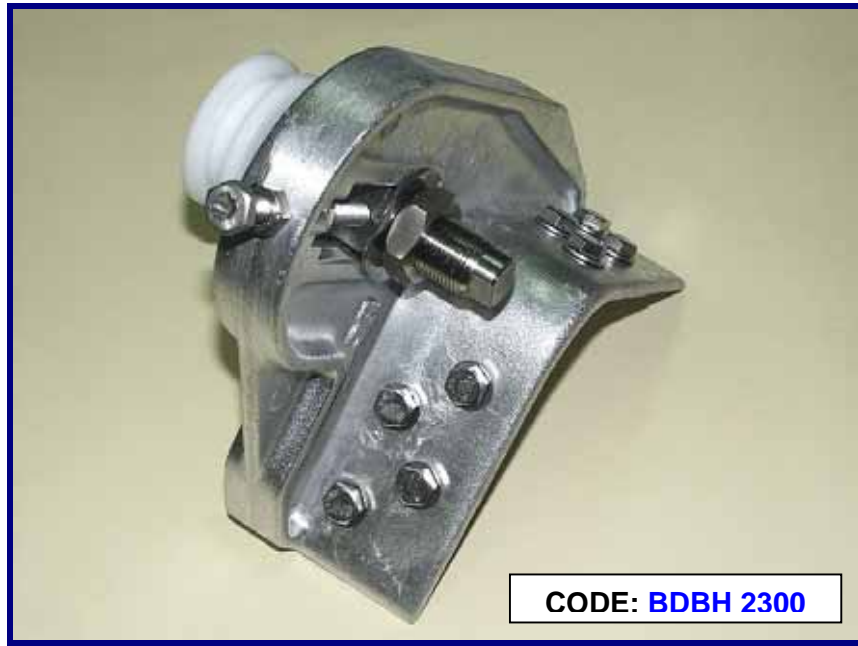
Wheel Bracket, BonDor, Door Hanger Roller Assembly, 55mm OD Wheel / Mill Finish, Stainless Steel Parts Available: Right or Left
