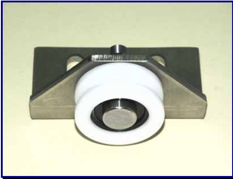
Wheel Bracket, Polyplas, Commercial Hanging Roller Assembly, 50mm OD Wheels Stainless Steel Parts All Parts Available Separately
